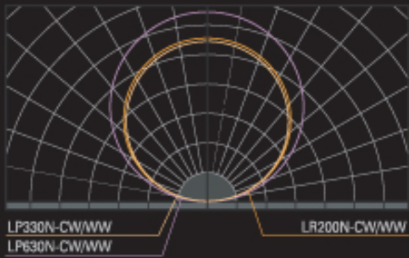
Distribution Curve of Luminous Intensity
